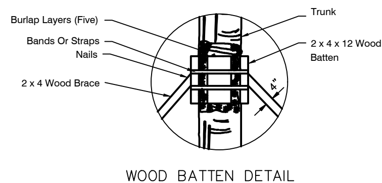
WOOD BATTEN DETAIL
