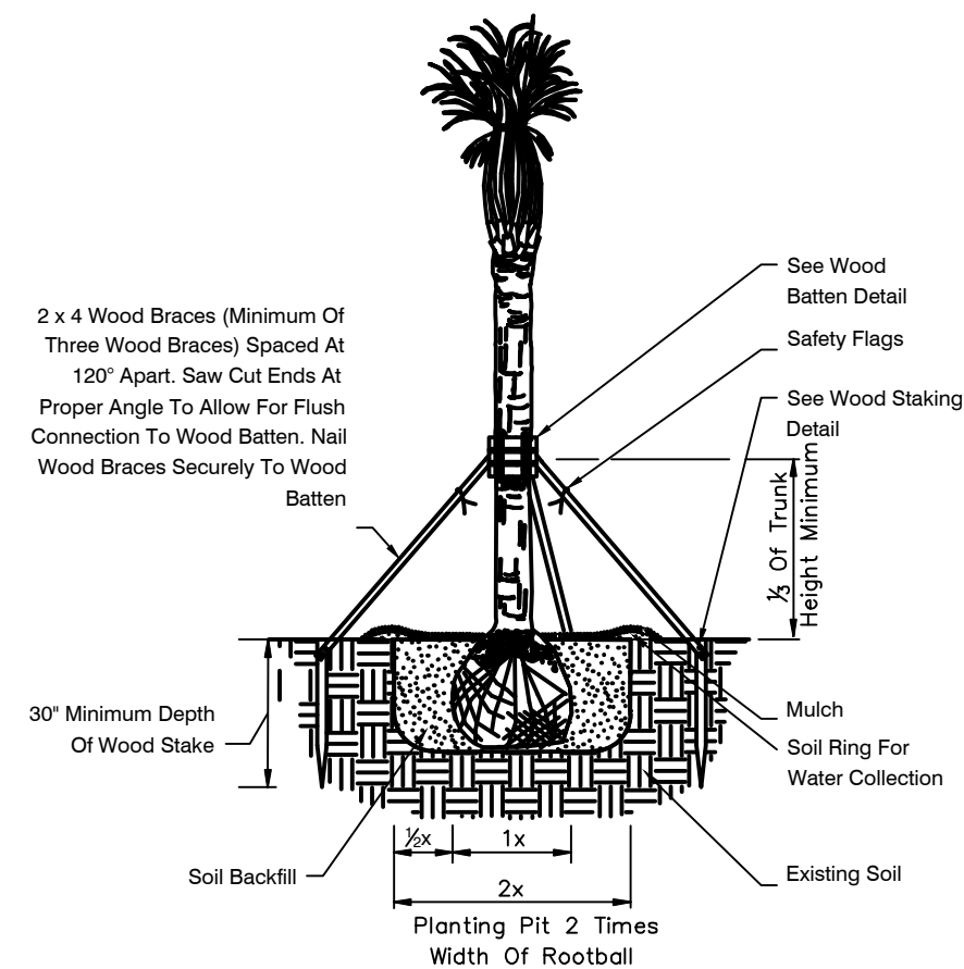
PALM PLANTING FOR UP TO 24' CLEAR TRUNK
