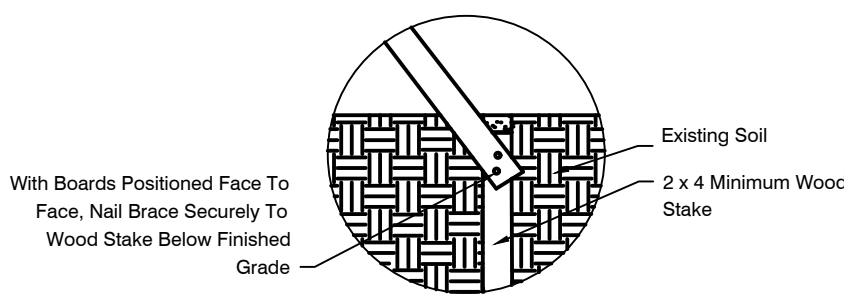
WOOD STAKING DETAIL
