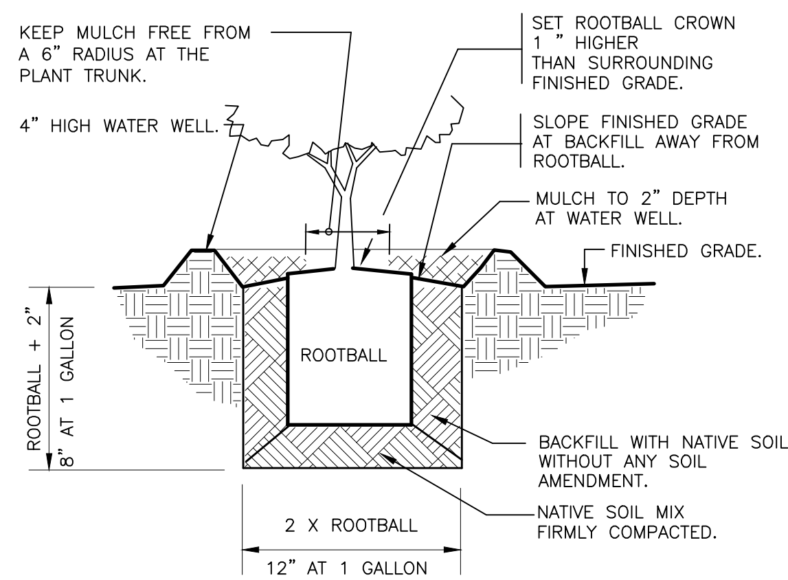
NATIVE SHRUB PLANTING
