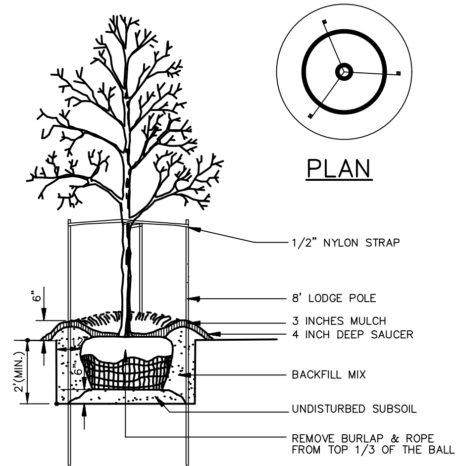
STAKING DETAIL
