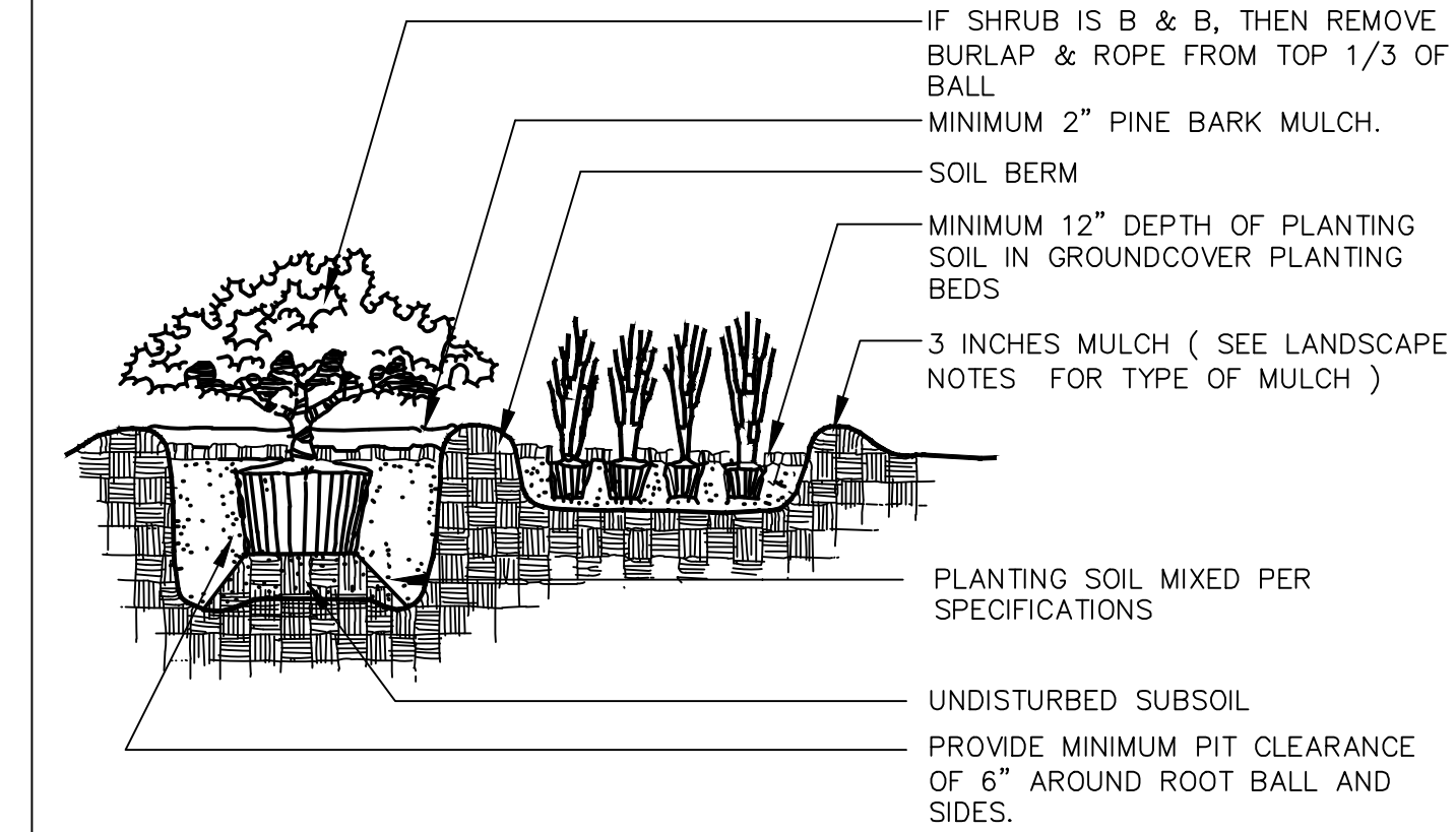
SHRUB AND GROUND COVER PLANTING DETAIL
